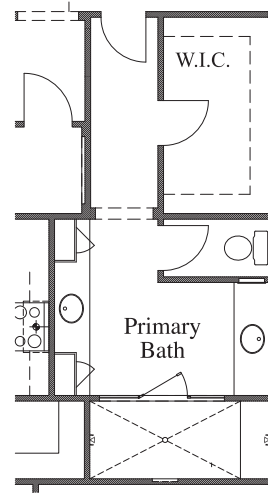
48 1/2 x 112" Mudset Shower at Primary Bath
