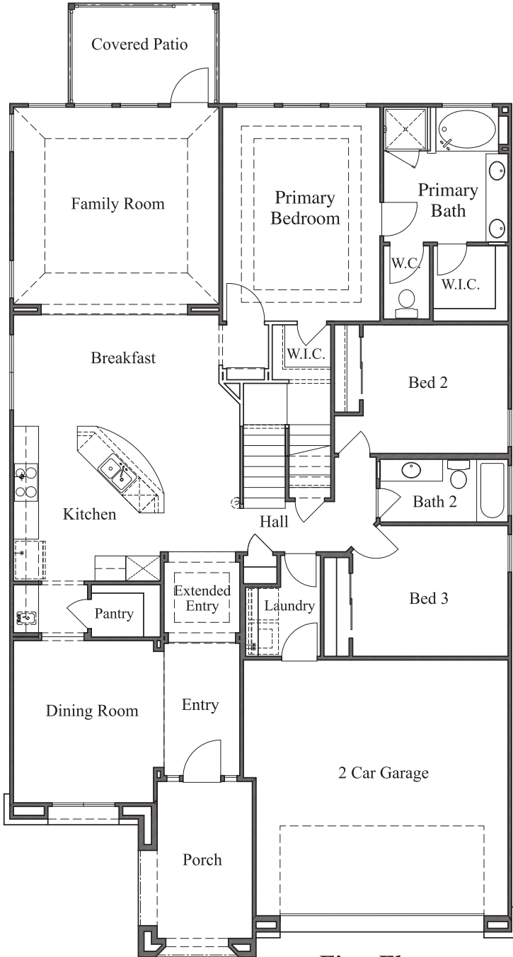
First Floor
